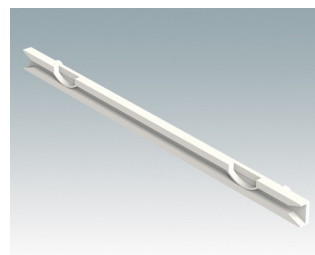
M6490020 Guide-carte, 140 mm PA 6/6 (UL 94 V-0) Fini naturel 139,7x7,5x3,5mm
