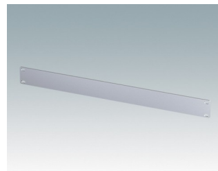
M6019010 Plaque avant 1Ux19" Aluminium Anodisé mat 482,6x3x43,6mm
