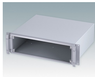
M5619335 UNIMET 19" 3Ux380mm Aluminium Gris clair/gris fenêtre RAL 7035/7040 132,5x482,6x380mm
