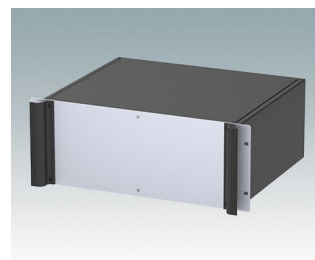
M6219459 COMBIMET 19" 4Ux365mm Aluminium Noir RAL 9005 177x482,6x365mm
